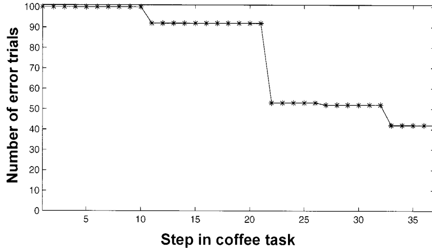
Figure 8. Survival plot for the coffee task under noise with variance 0.10. On the x -axis are steps in the sequence. The y -axis indicates the number of trials of 100 that remained error free at the corresponding step. Data are collapsed across the four versions of the task.
