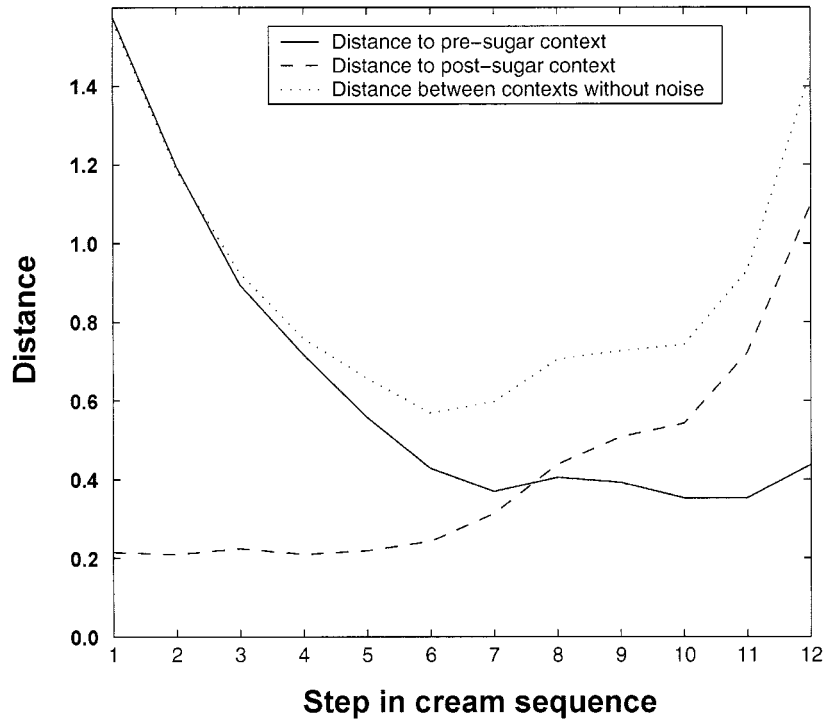
Figure 10. The steps of the cream-adding sequence leading up to a sugar perseveration error. The solid line represents the distance of the average context pattern from the presugar reference for the corresponding step. The dashed line represents the distance from the postsugar reference. The dotted line represents the distance between the two reference vectors. Data are based on averages across a sample size of 10.
