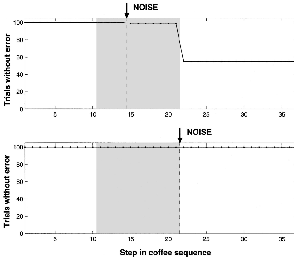
Figure 11. Survival plots based on 100 coffee-making trials with noise (variance = 0.50) applied at two points in processing. Dashed lines indicate points of noise injection. Steps belonging to the cream-adding subtask are indicated with gray shading. Top: Injection of noise at mid-subtask (before Step 15). Bottom: Injection of noise at subtask end (before Step 22).
