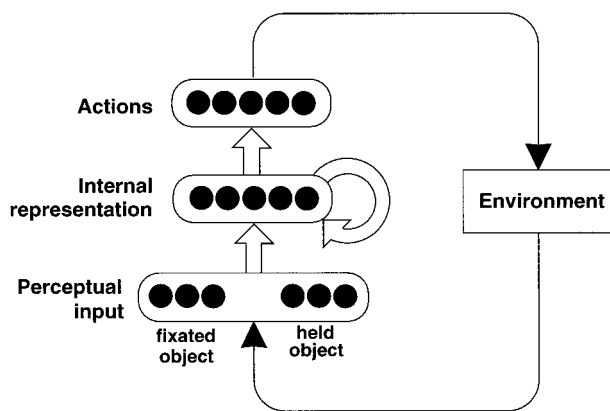
Figure 3. Architecture of the overall model. Open arrows indicate that every unit in the sending layer is connected to every unit in the receiving layer. (See text for details, including the number of units included in each layer.) From "Representing Task Context: Proposals Based on a Connectionist Model of Action," by M. Botvinick and D. C. Plaut, 2002, Psychological Research , 66, p. 300. Copyright 2002 by Springer. Adapted with permission.
