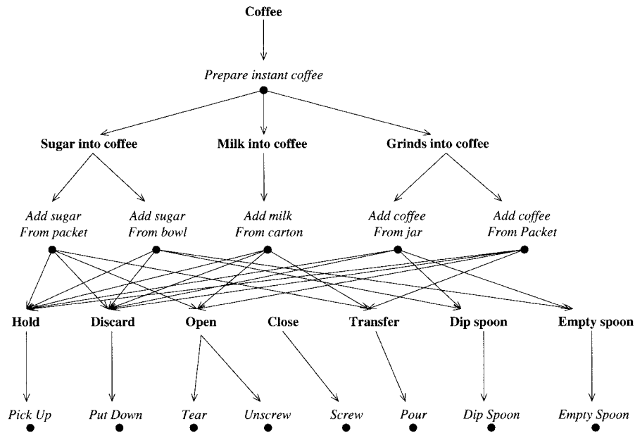
Figure 2. Processing architecture proposed by Cooper and Shallice (2000). From "Contention Scheduling and the Control of Routine Activities," by R. Cooper and T. Shallice, 2000, Cognitive Neuropsychology , 17, p. 307. Copyright 2000 by Taylor & Francis. Adapted with permission.
