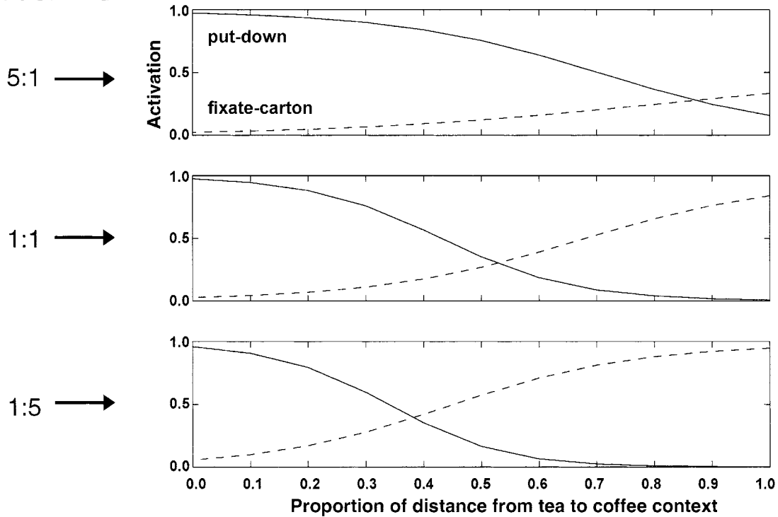
Figure 12. Effect on action selection of progressively distorting the context representation at the end of the sugar sequence in the tea task toward the corresponding coffee context. Ratios of tea to coffee during training were 5:1 (top), 1:1 (middle), and 1:5 (bottom).
