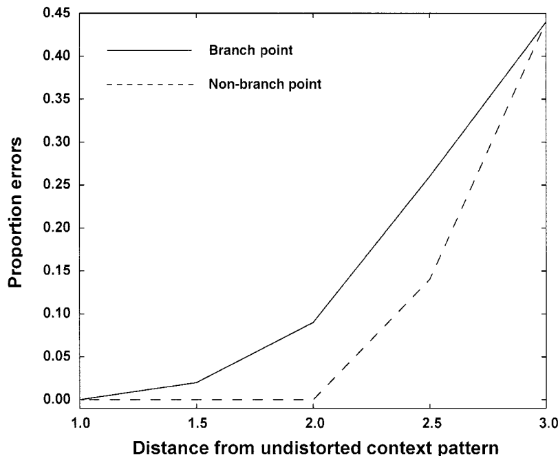
Figure 16. Greater distortion of context is needed to produce an incorrect action at a non-branch point than at a branch point. The data shown were produced by adding progressively increasing random noise to the context representations normally arising at a branch-point step (the first step of the DRINK subtask in the sequence GROUND → SUGAR (BOWL) → CREAM → DRINK; solid line) and a non-branch-point step (the peel-open step in the sequence GROUND → SUGAR (BOWL) → CREAM; dashed line) and observing the outputs produced by the network. The x -axis shows the Cartesian distance of the distorted context representations from the noise-free pattern (binned in steps of 0.5). The y -axis shows the proportion of trials on which the incorrect action was selected.
